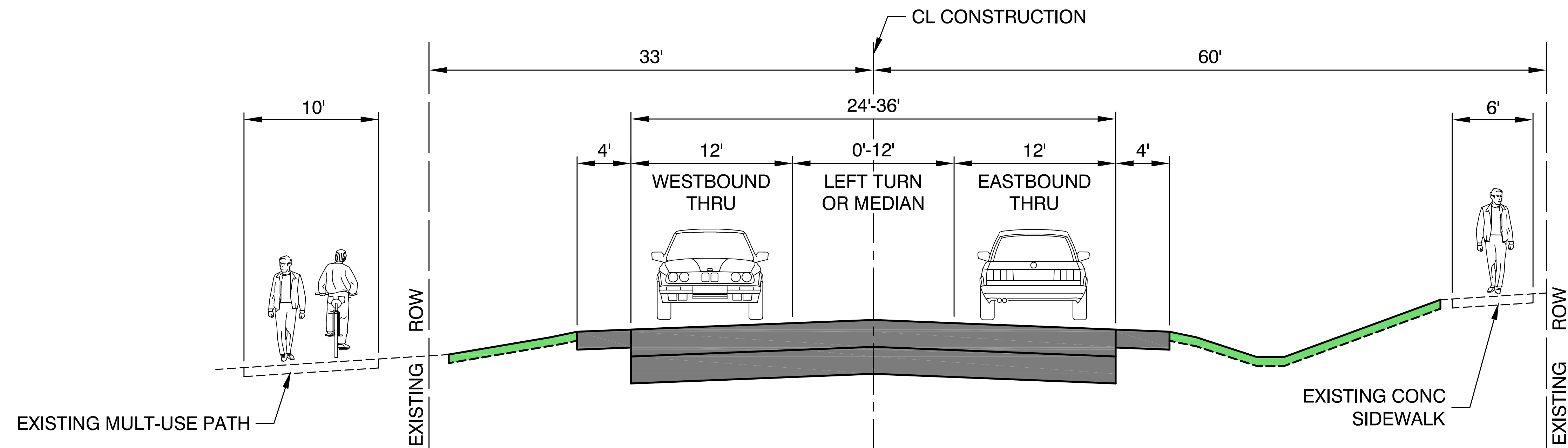
PROPOSED 175TH STREET RIDGELAND AVENUE TO HIGHLAND AVENUE
