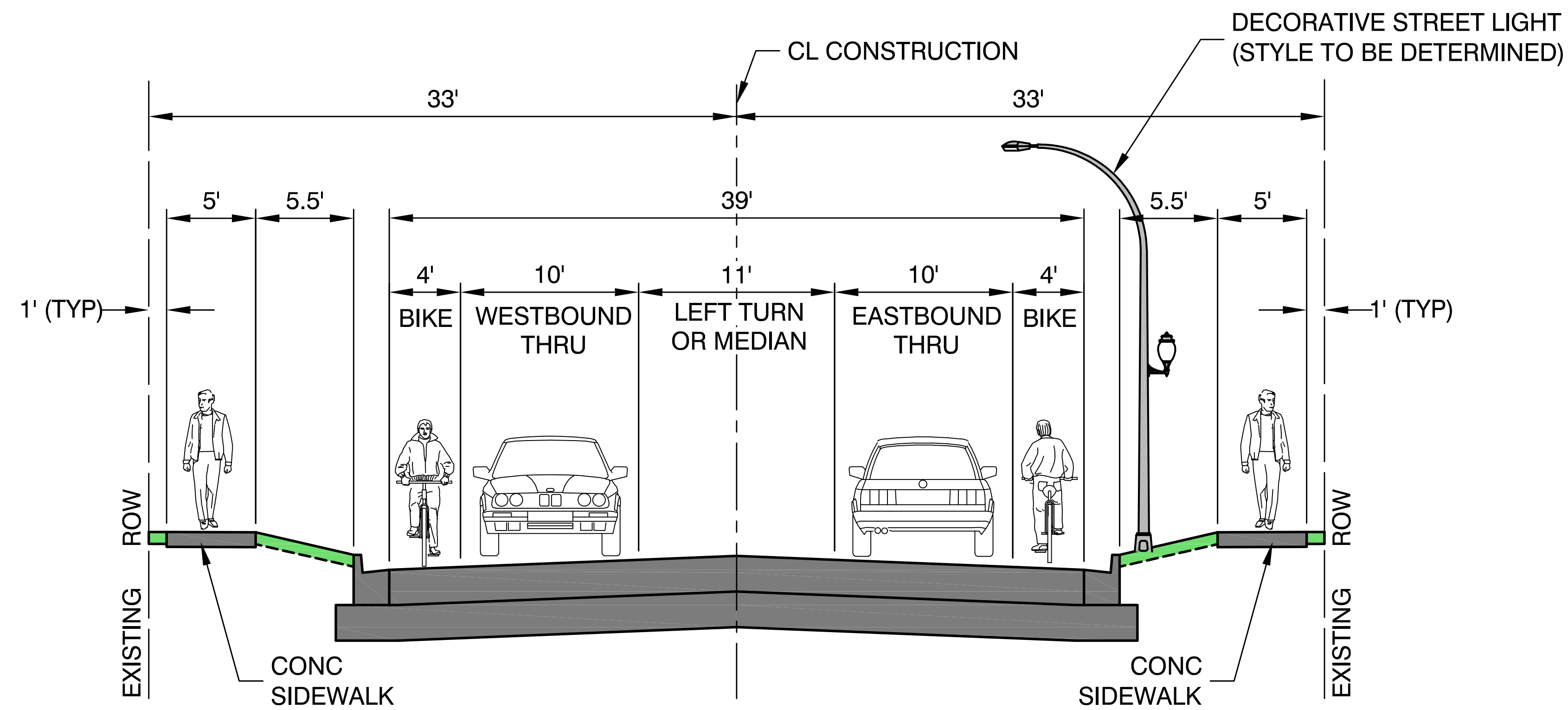
PROPOSED 175TH STREET OAK PARK AVENUE TO RIDGELAND AVENUE
