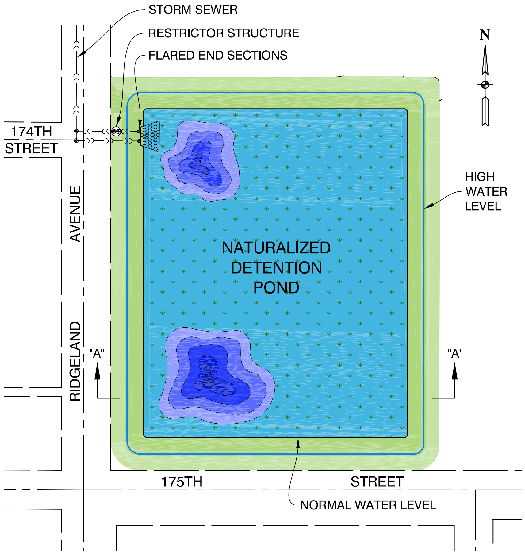
POND PLAN VIEW
